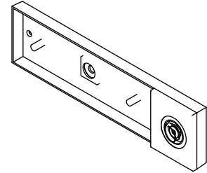
1511S TRIGGER & ARMATURE BASE 1511S-11
