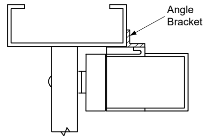
FIG. 2C Angle Bracket
