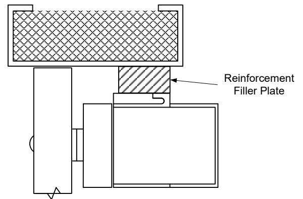
HOLLOW METAL CONCRETE FILLED FRAME
