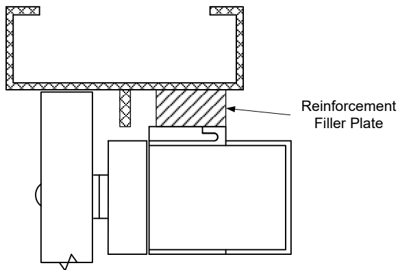
ALUMINUM FRAME WITH 1/2" BLADE STOP
