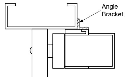
FIG. 2C With Angle Bracket
